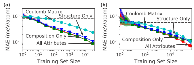
FIG. 6. Performance of ML models trained on different representations in cross-validation tests using data from the (a) ICSD subset of the OQMD and (b) the entire OQMD. These include models trained using all the attributes in our proposed representation and, separately, models created using only the composition-dependent terms and only the structure-dependent terms. The results of a model created using the Coulomb matrix representation with the random forest algorithm is shown for comparison. Shaded regions represent the 90% confidence intervals.
