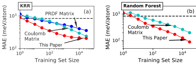
FIG. 3. Performance of ML models for formation enthalpy created with the same ML algorithm but different representations. Each graph shows MAE for (a) KRR model and (b) RF algorithm in a cross-validation test where the model was trained on progressively larger training sets and validated against a separate test set of 1000 entries. For each algorithm, we compare the performance using the Voronoi-tessellation-based representation proposed in this paper against the CM [30] and the PRDF [42] matrix representations.
