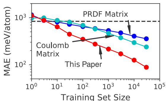
FIG. 1. MAE measured using cross validation of models created using the PRDF [42], CM [30], and the method presented in this paper. Each model was trained on the DFT formation energies of a set of randomly selected compounds from the ICSD and was used to evaluate 1000 distinct compounds that were also selected at random. The black, dashed line indicates the expected error from guessing the mean formation energy of the training set for all structures.
