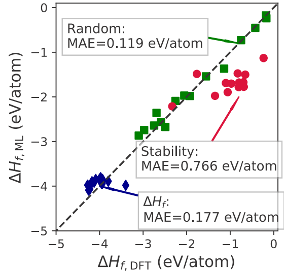
FIG. 7. Comparison of formation enthalpies ( \Delta H_f ) predicted using ML and computed using DFT. The ML model was trained on the formation enthalpies of all 435 792 nonduplicate entries from the OQMD. Each material was selected from a list of 12 667 entries from the ICSD that have yet to be included in the OQMD using three different strategies: (green squares) random selection, (blue diamonds) predictions with the lowest \Delta H_f , and (red circles) with the largest, negative difference between the predicted \Delta H_f and the OQMD convex hull.
