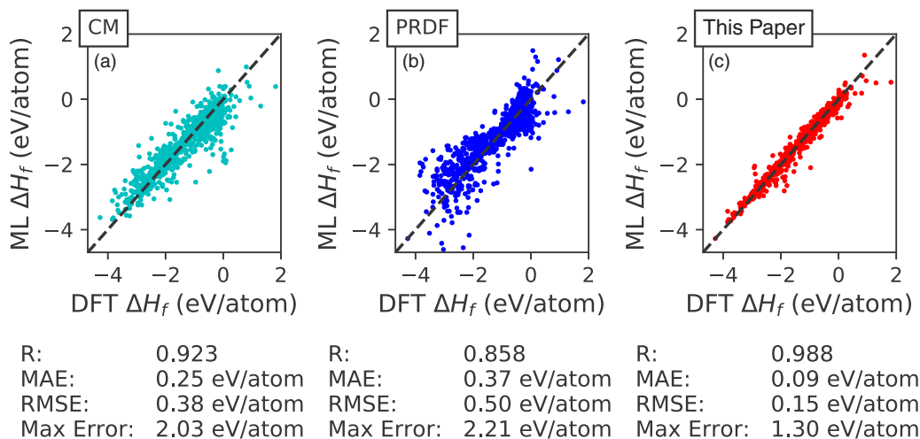
FIG. 2. Formation enthalpy ( \Delta H_f ) computed using DFT and predicted using ML with models created using the (a) CM [30], (b) PRDF [42], and (c) the method proposed in this paper. Each model was trained on the same set of 30 000 entries from the OQMD and evaluated against the same validation set of 1000 compounds. The results from the validation set are shown in this figure along with several different performance metrics.
