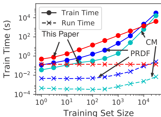
FIG. 4. Comparison of model training and running time of three different techniques to predict the formation energy of inorganic compounds: Coulomb Matrix (CM) [30], Partial Radial Distribution Function (PRDF) [42], and our Voronoi-tessellation-based method. Training time is the sum of attribute generation and model construction with given data. Run time is the average time taken to compute the required attributes and to evaluate the ML model for a single compound.
