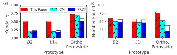
FIG. 8. Comparison of the ability of different ML methods to rank different types of compounds based on DFT formation energy, measured using two different metrics. (a) The Kendall \tau ranking correlation coefficient, which is based on how well the model ranks the entire dataset. A correlation value of 1.0 corresponds to perfect ranking. (b) The number of the 100 compounds with the lowest DFT formation energy that were predicted by the model to be within the lowest 100 compounds. Each model was trained on the DFT-predicted formation energy of 32 111 inorganic compounds from the ICSD. The solid bar indicates the ranking performance using the input structure provided to DFT. Black outline around each bar indicates the ranking accuracy when provided with the fully relaxed output from DFT.
