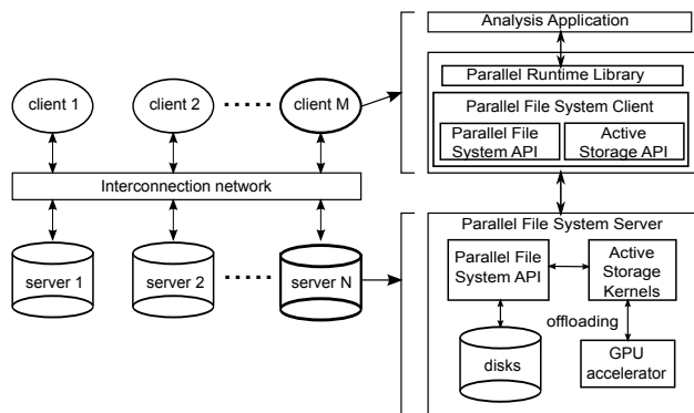
Fig. 3. Overview of our active storage system and our default storage deployment architecture. There are M clients connected to N active storage nodes.
