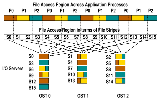
Fig. 2. File access region is partitioned among the application processes P_0, P_1, and P_2 . Different colors represent data accessed by different application processes. From Lustre file system’s perspective, the entire file is partitioned into 16 stripes S_0, S_1, \dots, S_{15} which are distributed across the I/O servers, OST_0, OST_1, and OST_2 . Even though file accesses are nonoverlapping among the processes, when requests from two processes access the same stripe, lock conflict occurs.
