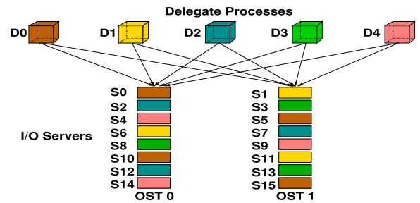
Fig. 5. If delegate processes are not a factor or multiple of I/O servers then all the delegate processes might be accessing all the I/O servers causing serious lock acquisition competition between the processes. In this example, each I/O server is contended by all the delegates which may deteriorate I/O performance.
