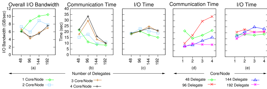
Fig. 7. S3D I/O Kernel, 2,048 application processes, Franklin: Breakdown analysis of two major time consuming operations: (i) Data Communication between application and delegate processes. (ii) File system I/O. (a)-(c). Overall I/O bandwidths, time spent in data communication among the application and delegate processes, and file system I/O time as a function of number of delegates, respectively. (d) and (e). Time spent in data communication among the application and delegate processes and time for file I/O with varying number of cores-per-delegate-node, respectively.
