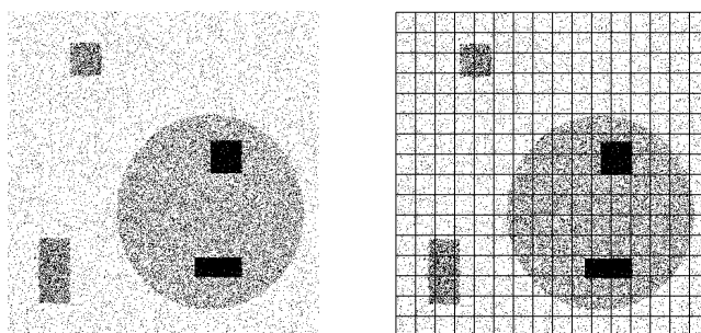
Figure 1: (a) An example of data distribution with nested clusters. (b) A single uniform mesh is applied to the spatial domain, which may not be sufficient for good quality clustering.
