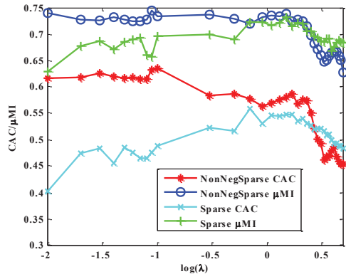
Fig. 3. The changes of cluster performance criteria w.r.t. the \lambda (in log scale).
