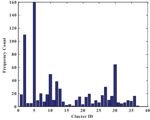
Fig. 2. The number of images in each of the 37 clusters.
