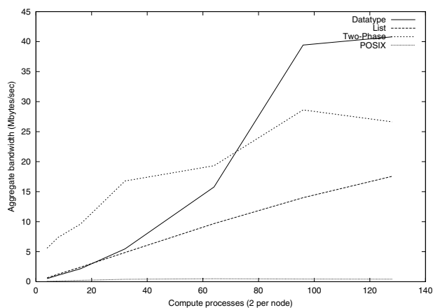
Figure 12. FLASH I/O Performance
